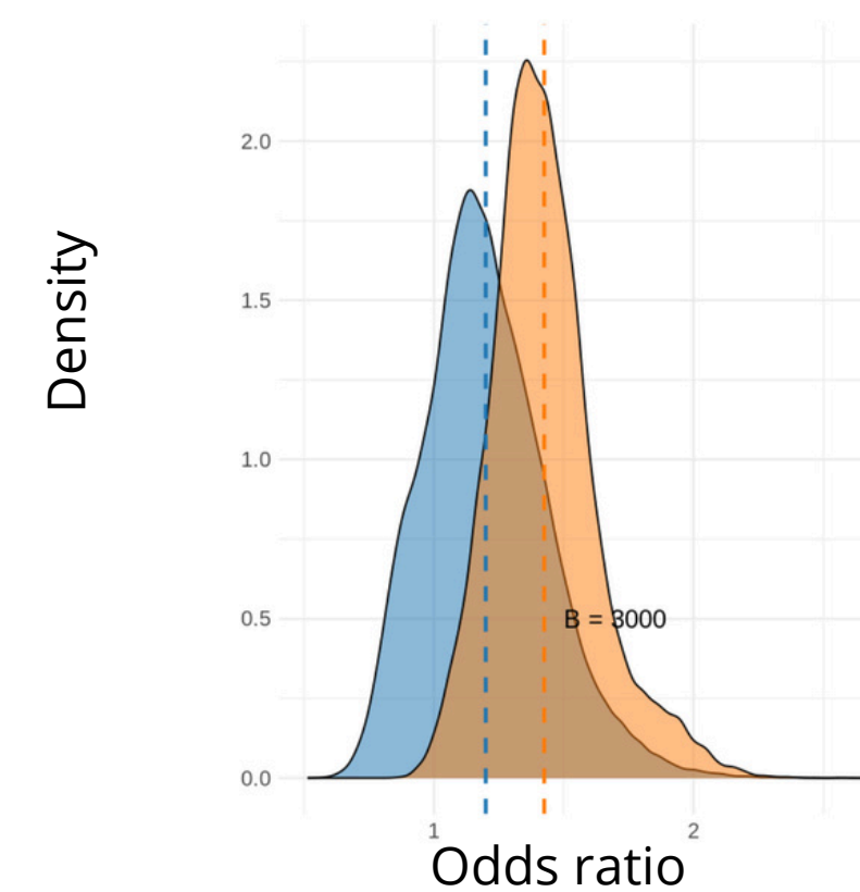
OPENNESS TO EXPERIENCE
